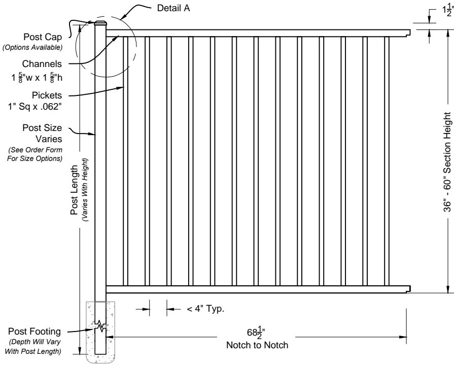
01 Alamo #400 6ft Fence Panel Shown As Industrial Series Scale: NTS
