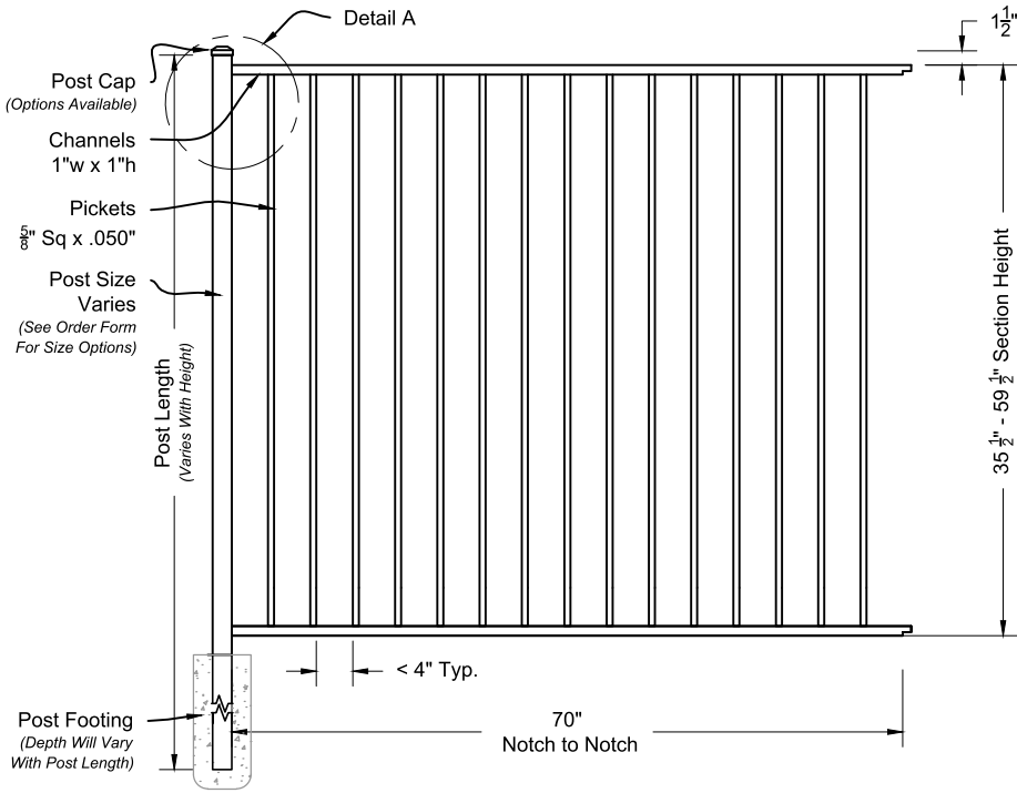
i 01 Alamo #400 6ft Fence Panel Shown As Residential Series Scale: NTS
