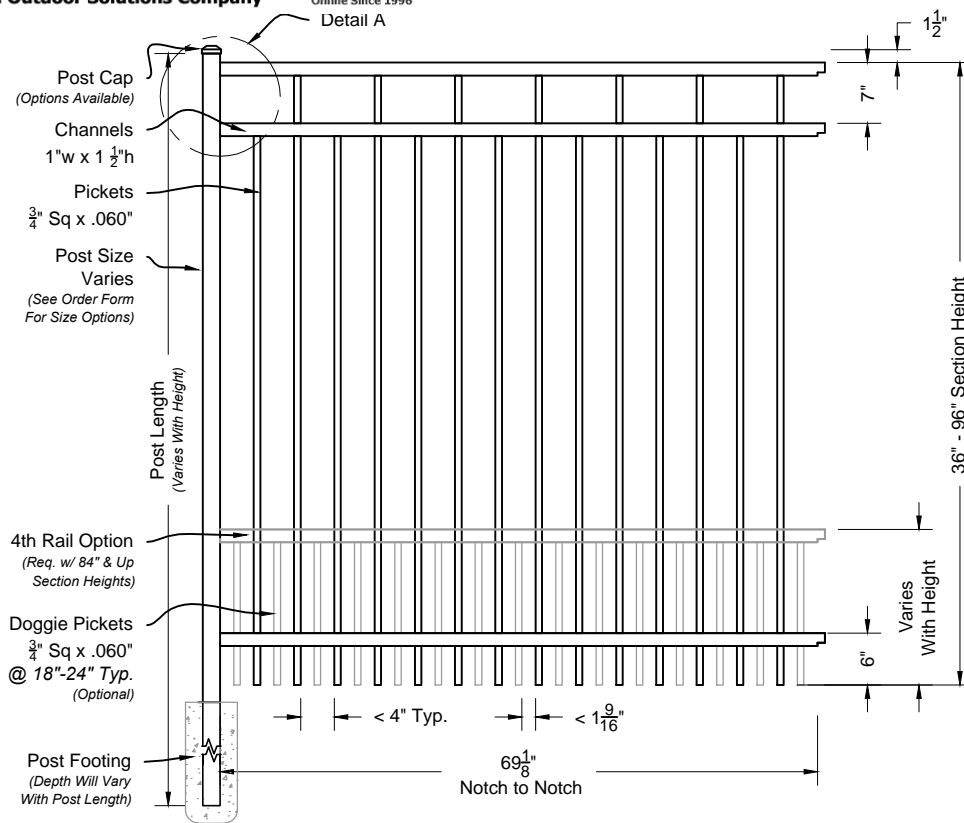
i 01 Carolina #403 6ft Fence Panel Shown As Commerical Series Scale: NTS
