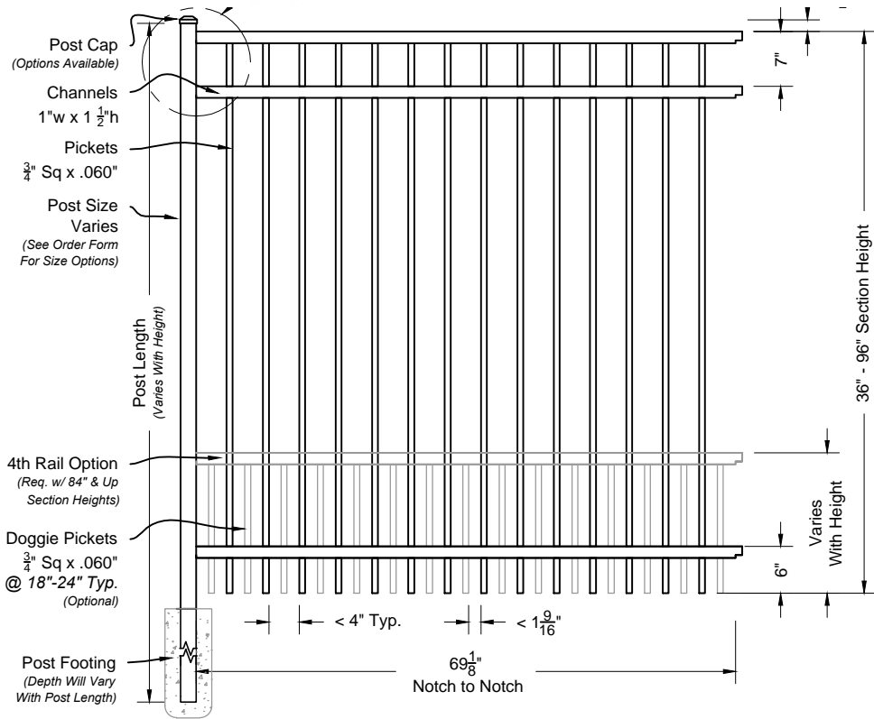
01 Long Islander #300 6ft Fence Panel Shown As Commercial Series Scale: NTS
