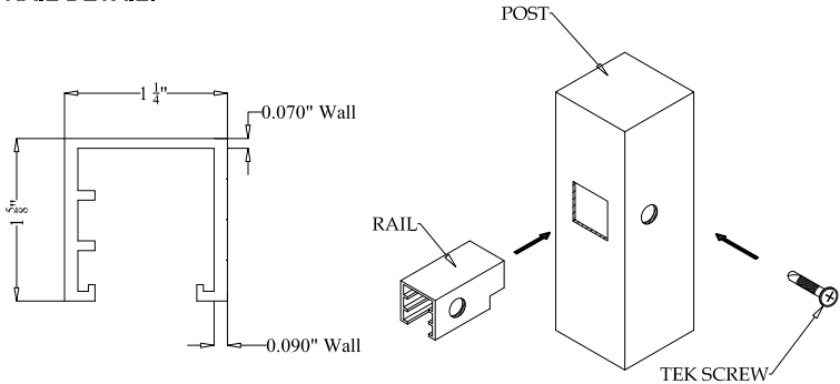
COMMERCIAL RAIL
