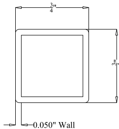
COMMERCIAL PICKET
