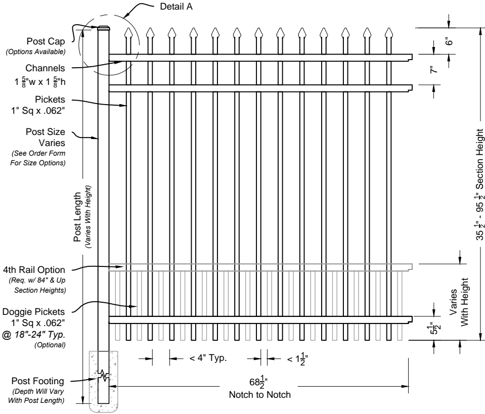
i 01 Maine #203 6ft Fence Panel Shown As Industrial Series Scale: NTS
