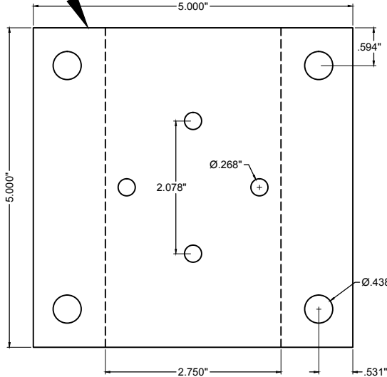
Front Elevation View
