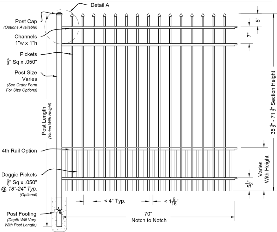
01 Maine #203 6ft Fence Panel Shown As Residential Series Scale: NTS
